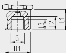
EN 837, female thread
