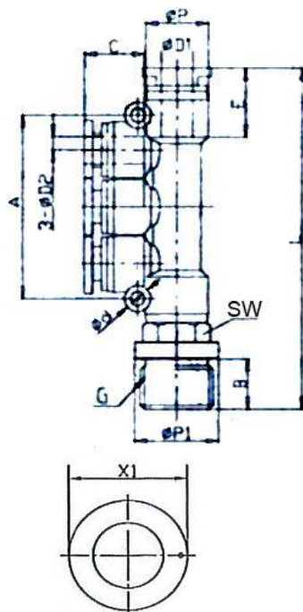
Tee distributor with parallel male thread, with O-ring, swivel type
