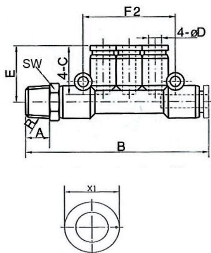
Tee distributor with conical male thread, coated, swivel type
