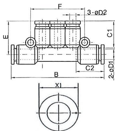
Tee distributor with plug connection, 3 unequal outlets
