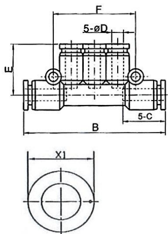
Tee distributor with plug connection
