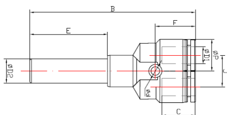
Y union with push-in plug, unequal
