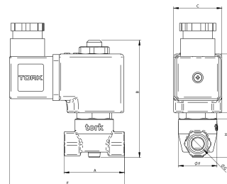
Dimensions (mm)
