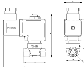
Dimensions (mm)
