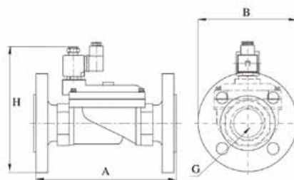
Dimensions (mm)
