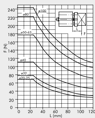
TRANSVERSAL FORCE FOR NON-ROTATING THROUGH-ROD
