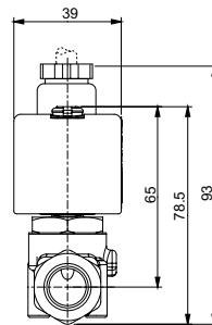
① 2 mounting holes: 190-24 UNC-2B, depth 6 mm
